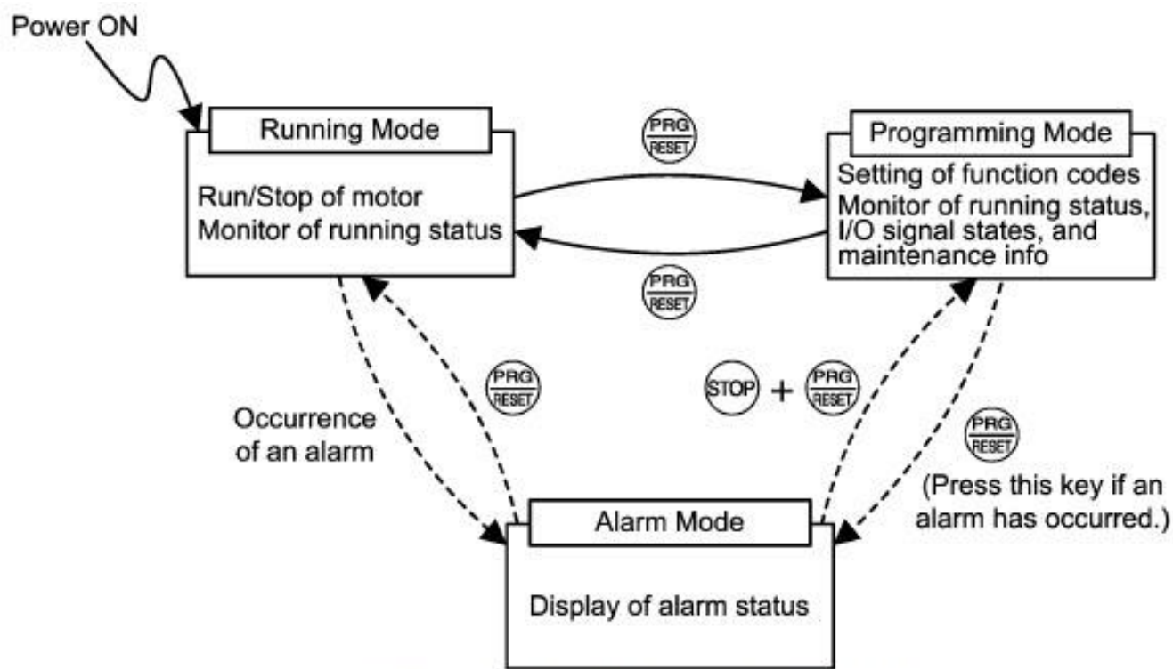
Status Transition between Operation Modes
