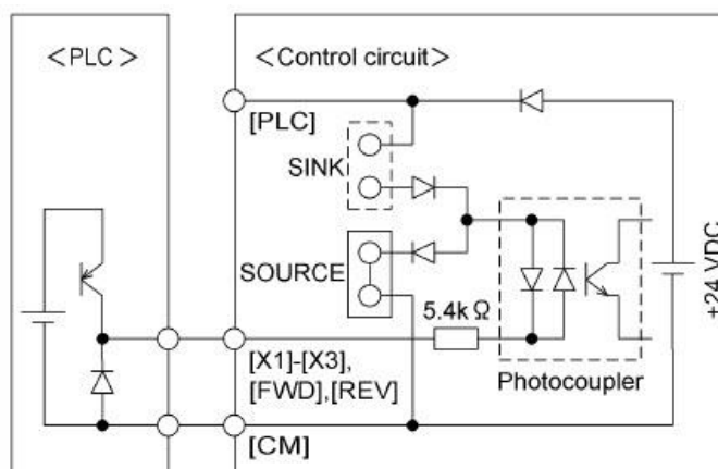
(b) With a jumper applied to SOURCE
