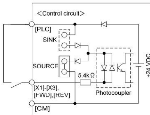
(b) With a jumper applied to SOURCE.
